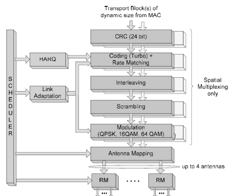
Figure 5 – Signal generation chain in LTE
