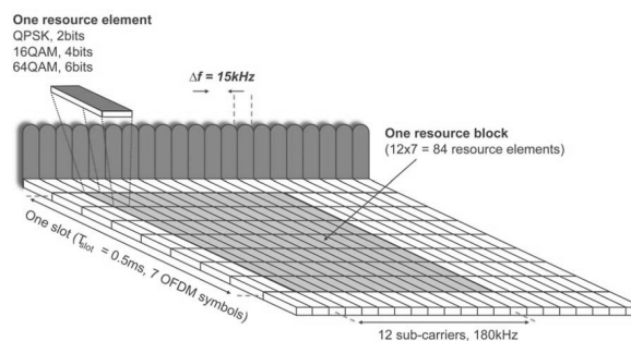
Figure 6 – Two dimensional resource management in LTE
