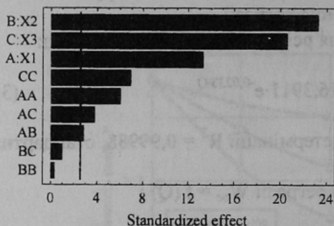
Standardized Pareto Chart for q
