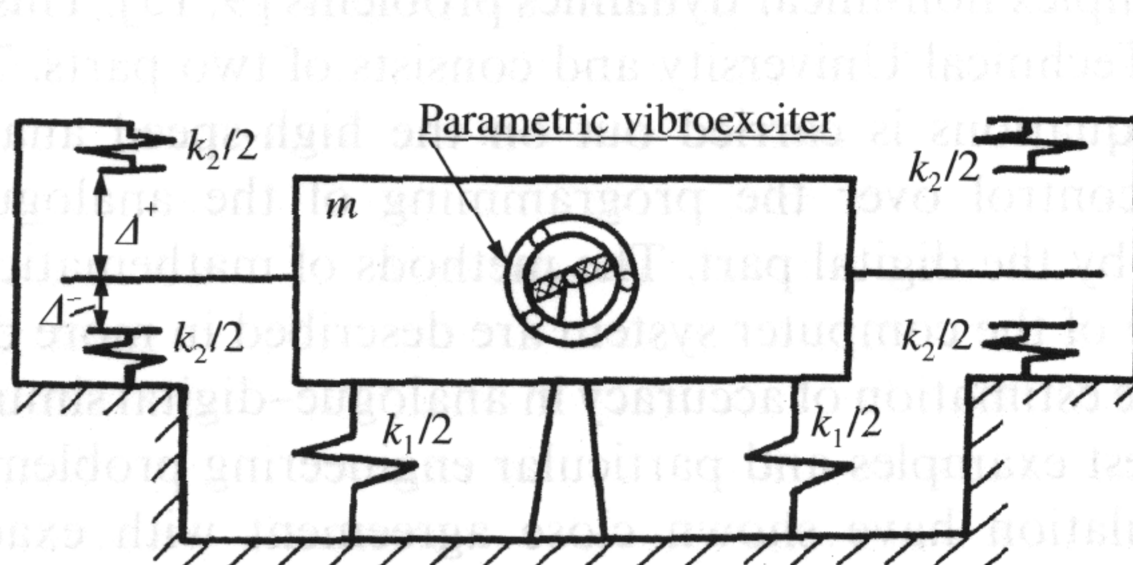
Figure 2. Vibromachine model considered in the dynamic analysis.
