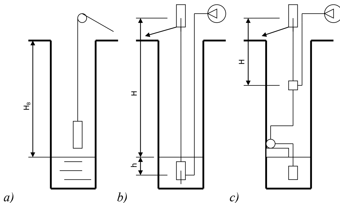
Figure 1 - Circuits of drainage of ventilating shafts: a) - with use tub; b) - эрлифтом; c) - pump -airlift installation
