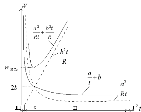
Fig. 2. Determination of the minimal energy of excitability of structures
