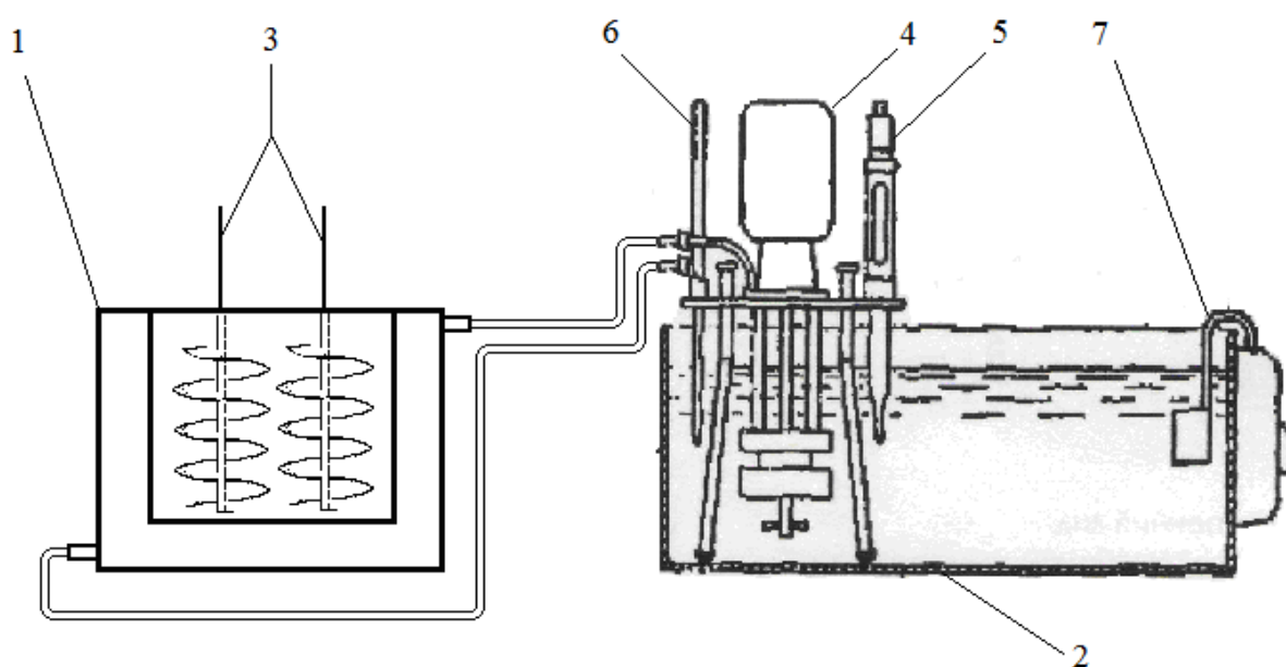
Figure 1. The scheme of experimental plant for compositional materials obtaining based on modified coal tar pitch: 1 - jacketed reactor, 2 – thermostat, 3 - screw mixers, 4 - pump, 5 - contact thermometer, 6 - controlling mercury thermometer, 7 – electric heating element
